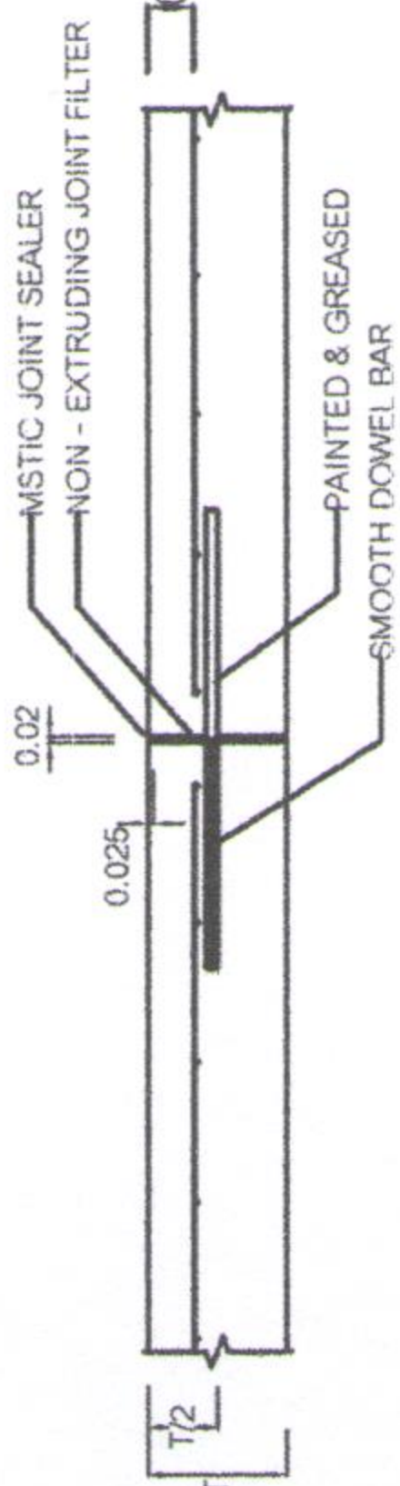
EXPANSION JOINT
